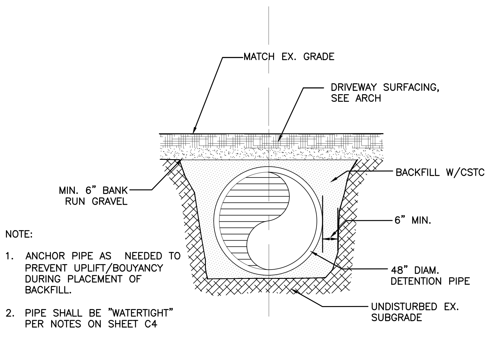
2 DETENTION PIPE DETAIL C3 NTS
